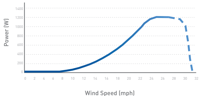
Power Curve
