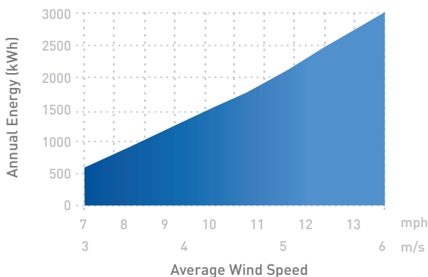
Annual Energy Production
